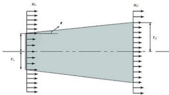
Fig. 1 Jensen wake model
