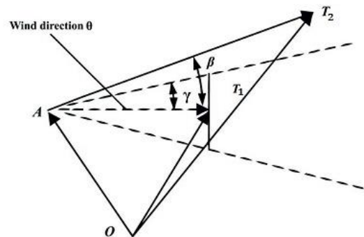
Fig. 2 How to put a turbine in the cone of another turbine speed and display the angles in Formula (9) [8]
