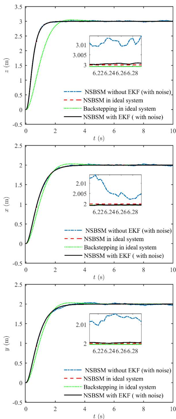
Fig. 4 Tracking results for the position (z, x, y)
