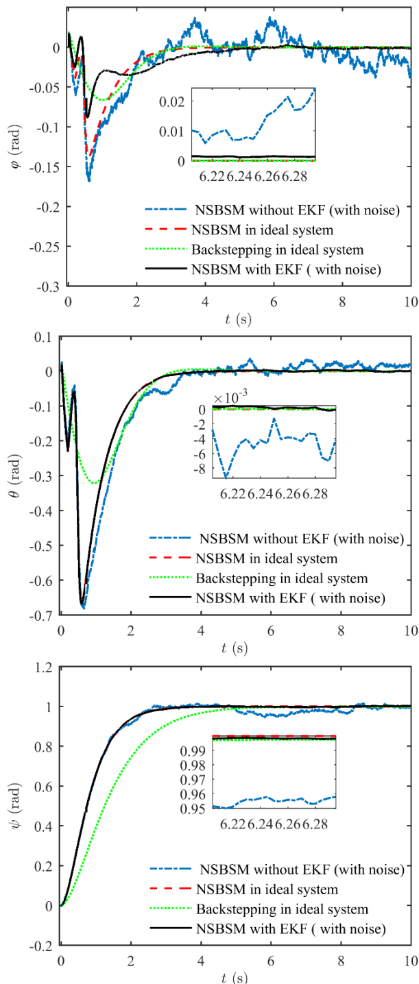
Fig. 3 Tracking results for the orientation (\varphi, \theta, \psi)
