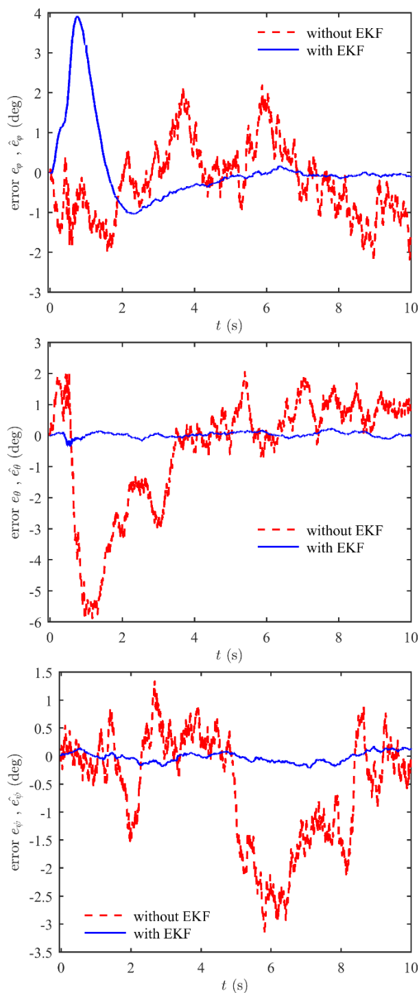
Fig. 5 Tracking errors results for the orientation (\varphi, \theta, \psi)
