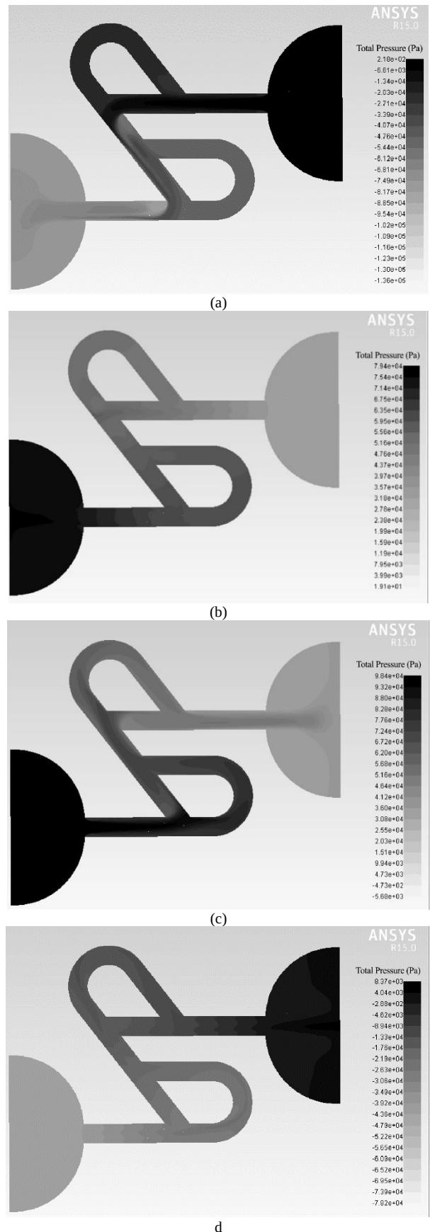
Fig. 13. Pressure contours at Re = 425 and f = 1000\text{Hz} at different times: a) t = 0.002\text{s} , b) t = 0.00225\text{s} , c) t = 0.0025\text{s} , d) t = 0.00275\text{s}
