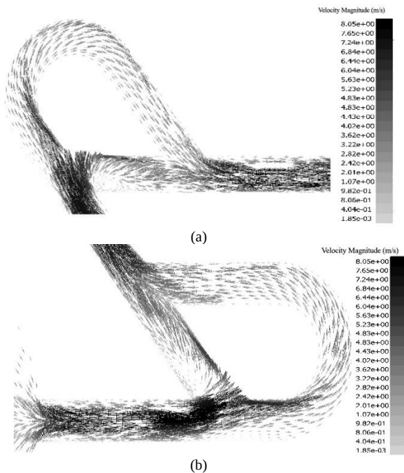
Fig. 11. The velocity vectors at the conjunctions at Re=426 and f=1000\text{Hz} in the transition state ( t=0.0025\text{ s} ): a) location C and D, b) location A and B
