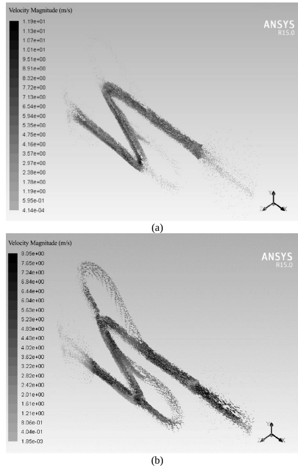
Fig. 10. Three-dimensional velocity vectors at Re=426 and f=1000\text{Hz} at different times: a) backward ( t=0.002\text{s} ), b) forward ( t=0.0025\text{s} )
