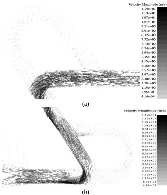
Fig. 12. The velocity vectors at the conjunctions at Re=426 and f=1000\text{Hz} in backward mode ( t=0.002\text{s} ): a) location C and D, b) location A and B
