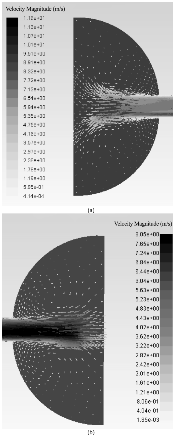
Fig. 9. Velocity vectors at the valve output at Re=426 and f=1000Hz at different times: a) the Backward ( t=0.002s ), b) Forward ( t=0.0025s )
