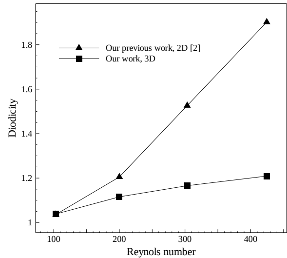
Fig. 6. Diodicity as Reynolds number in steady 2D and 3D simulations
