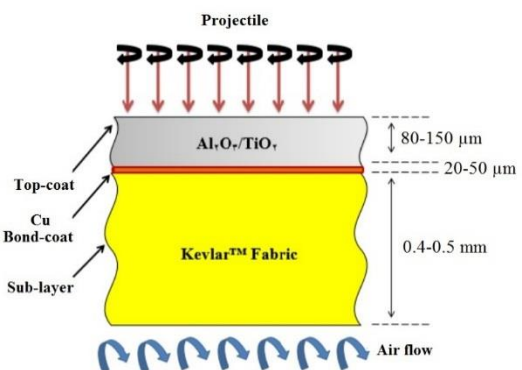
Fig. 1 Schematic image of the applied coating.
