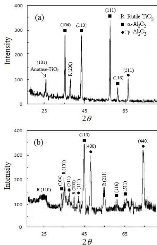
Fig. 9 XRD pattern for: a- \text{Al}_2\text{O}_3/13\text{wt.}\text{TiO}_2 powder, b- coated sample.
