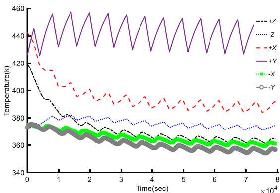
Fig. 9 Temperature variation curve for six surfaces after 28 steps
