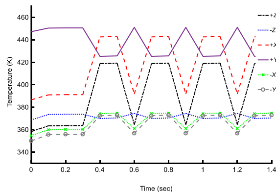
Fig. 8 Temperature variation curve for six surfaces after 1 step
