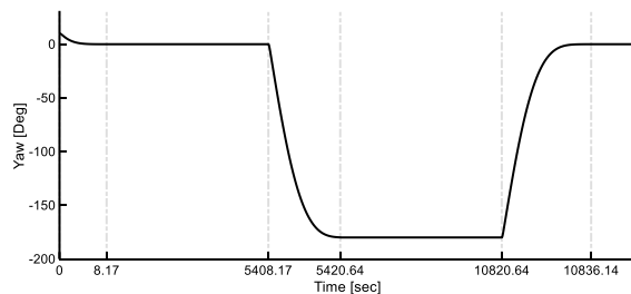
Fig. 10 Yaw angle variation curve using integrated control system
