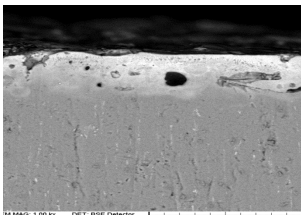
Fig. 6 SEM micrograph showing cross-section of EDAed piece (1000X)
