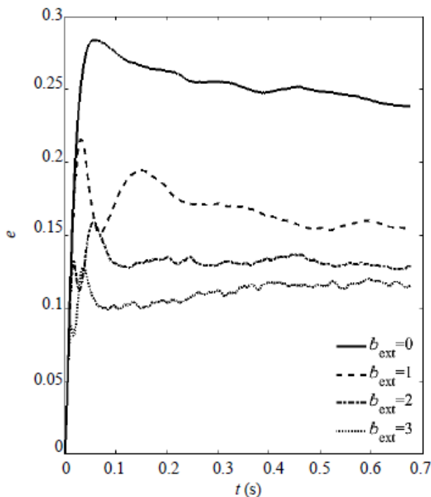
Fig. 5 Mixing efficiency changes of flow with external magnetic field b_y = 0, 1, 2, 3
