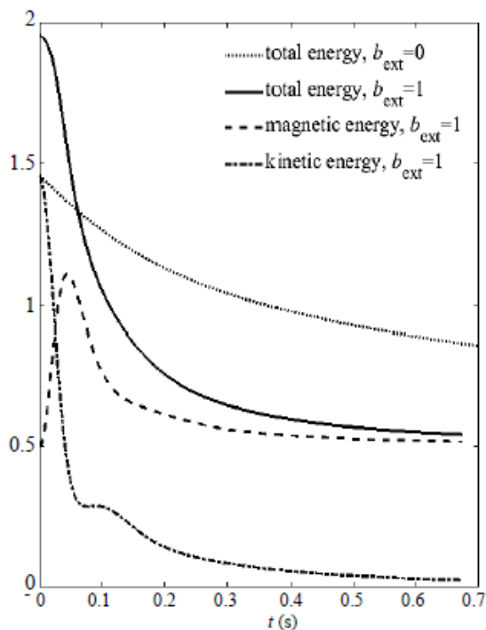
Fig. 8 Total energy and energy transfer between the kinetic and magnetic components in MHD
