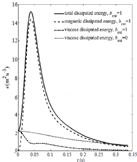
Fig. 7 Total, viscose & magnetic dissipated energy rate
