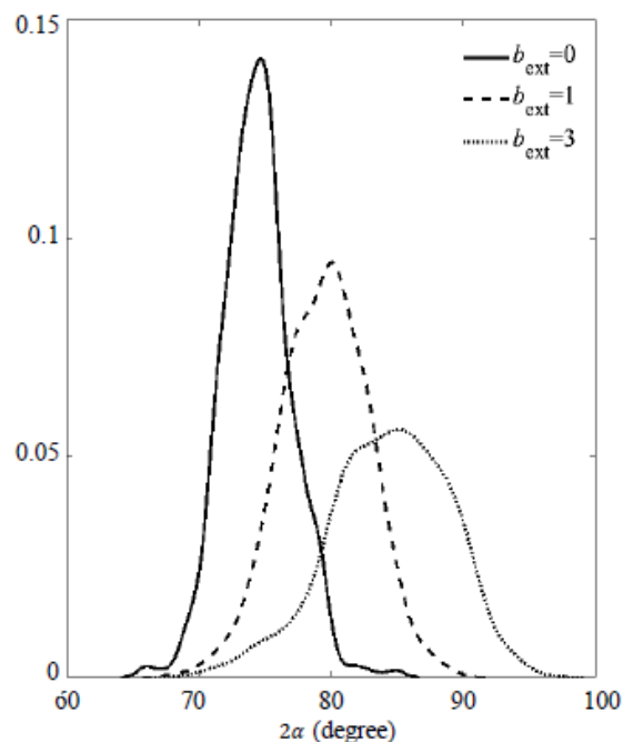
Fig. 6 The probability density function of 2\alpha with external magnetic field ( b_y = 0, 1, 3 )
