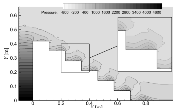
Fig. 8 The contour lines of static pressure (Pa) obtained with VOF model for no air intake geometry Q=45\text{lit/s.m}
