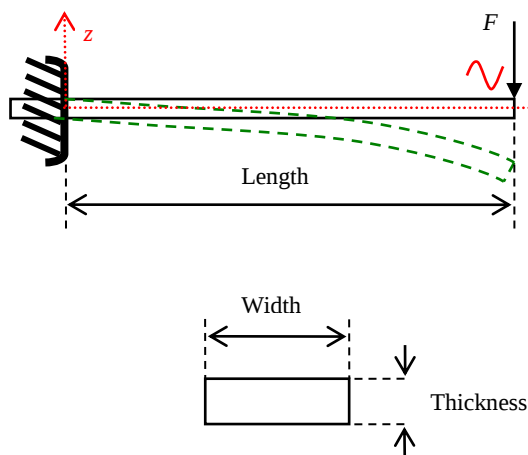
Fig. 1 SMA Cantilever beam
