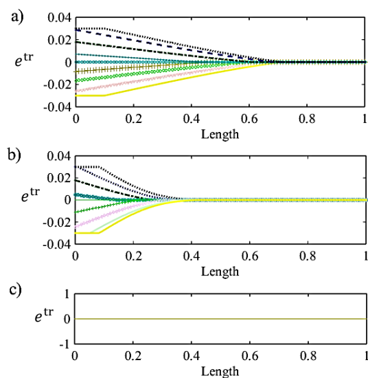
Fig. 9 Transformation strain in layers of cross section a) t=0.02 b) t=1.57 c) t=47.5
