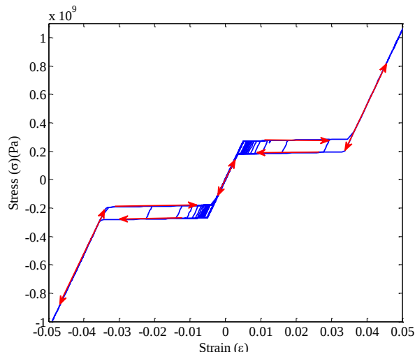
Fig. 5 Strain-Stress diagram for top point on clamped end
