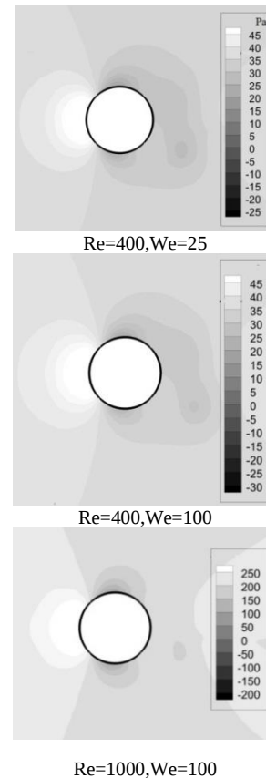
Fig. 8 Distribution of pressure (Pa) around the sphere on y=0 plane at t=0.11s
