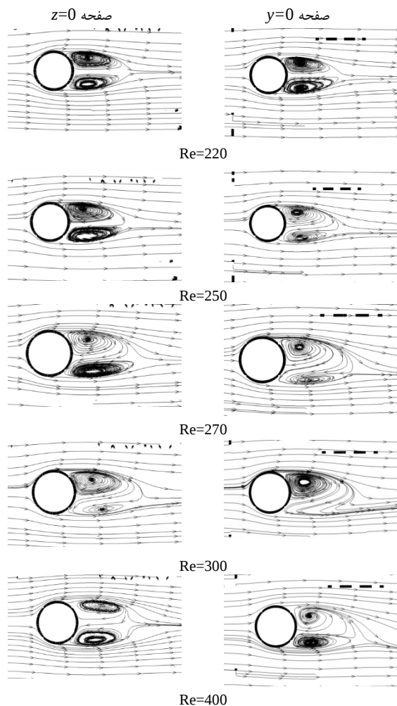
Fig. 3 Streamlines around sphere versus Reynolds number on xy and xz planes
