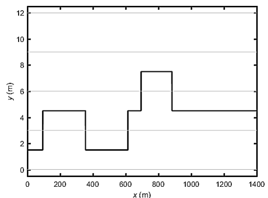
Fig. 7 The primary path produced from time interval method
