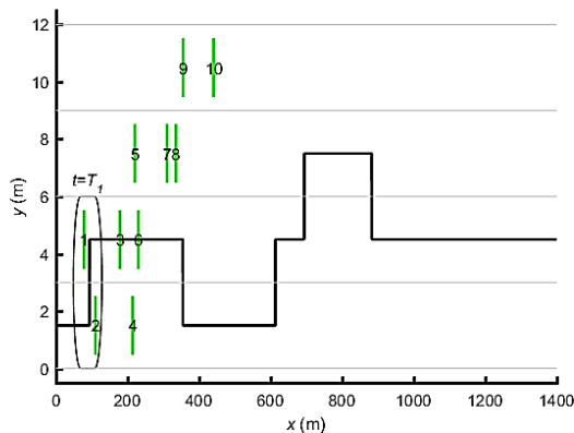
Fig. 8 Obstacles positions at t=T_1 and the path in that moment
