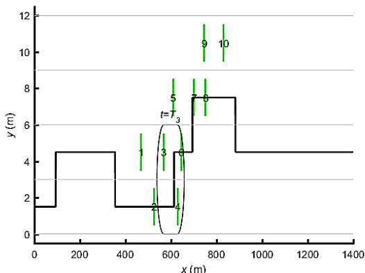
Fig. 10 Obstacles positions at t=T_3 and the path in that moment
