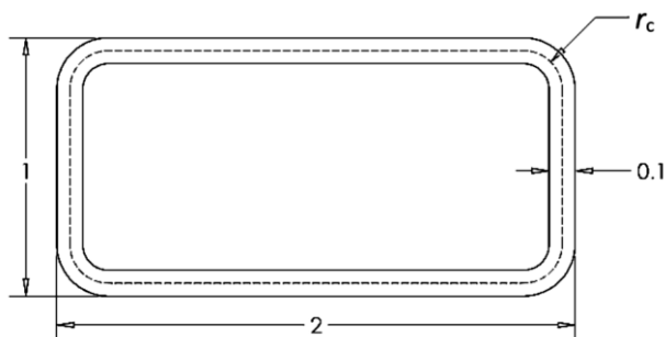
Fig. 2 A hollow rectangular section with rounded corners
