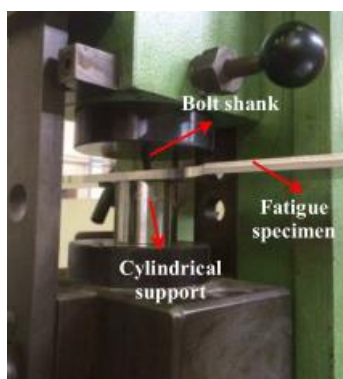
Fig. 3 Interference fit set up
