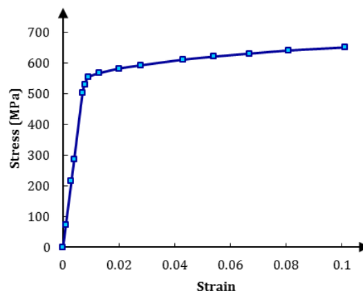
Fig. 1 Stress- strain curve of Al- alloy 7075-T6
