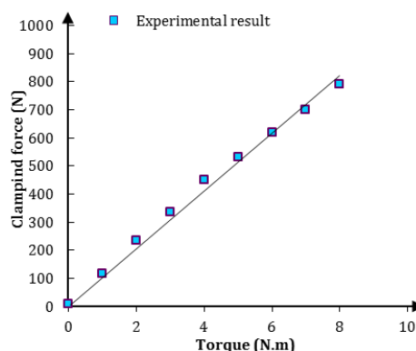
Fig. 5 Linear relation between tightening torque and bolt clamping force.
