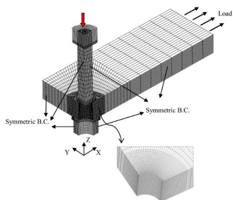
Fig. 12 Finite element model
