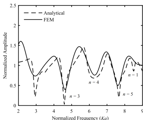
Fig. 9 The normalized backscattered spectrum of the embedded steel cylinder in epoxy matrix
