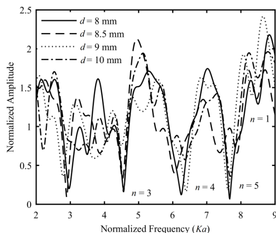
Fig. 11 Variation of the backscattered spectrum from a grating of two adjacent cylindrical fibers with change of center-to-center distance of fibers
