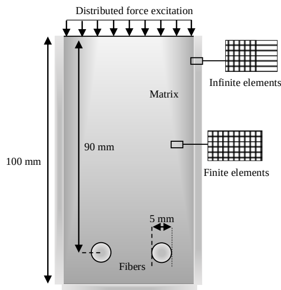
Fig. 10 Schematic configuration of the wave scattering problem from two adjacent cylinders
