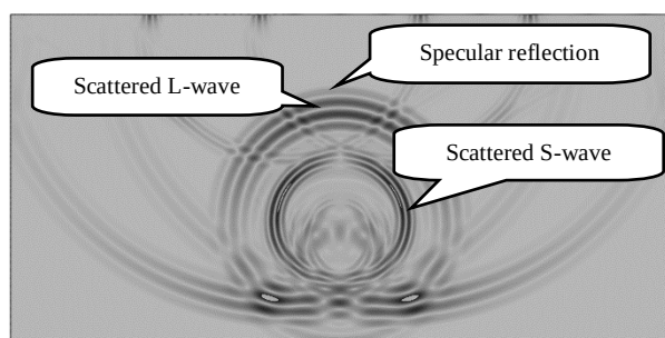
Fig. 6 Ultrasonic wave scattering from steel cylinder embedded in epoxy matrix
