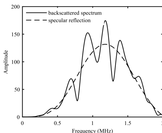
Fig. 8 Frequency spectra of the backscattered signal and the corresponding specular reflection
