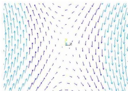
Fig 10 Velocity vectors near the hyperbolic point
