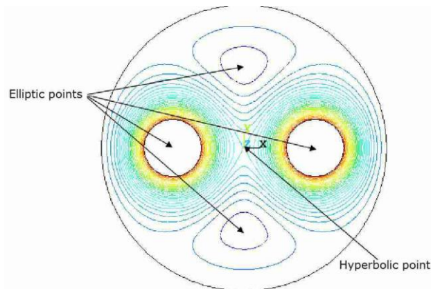
Fig 9 Streamline inside the mixer in mode 1 (constant rotor speed)
