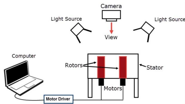
Fig 3 Schematic of the chaotic mixing flow apparatus
