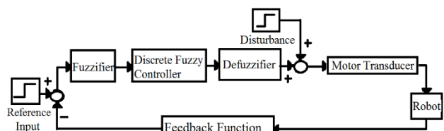
Fig. 5 Fuzzy controller simulation in Simulink
