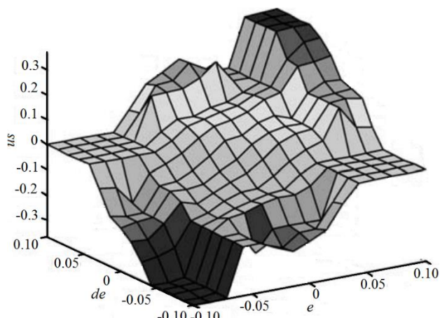
Fig. 4 The fuzzy surface for the system[3]
