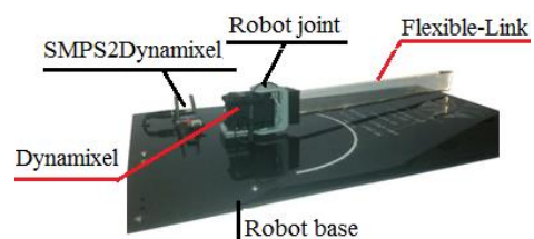
Fig. 1 Single flexible-link robot made in laboratory
