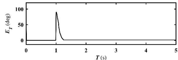
Fig. 20 Position error for fractional order PID torque control in presence of disturbance
