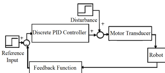
Fig. 2 PID controller simulation
