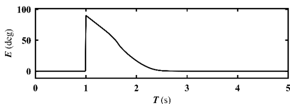
Fig. 10 Position error for fuzzy controller
