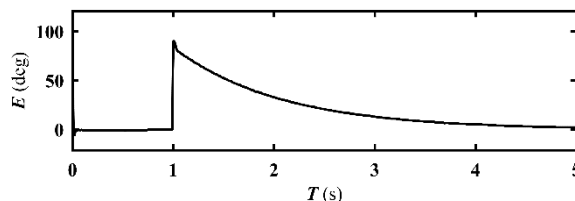
Fig. 8 Position error for PI controller
