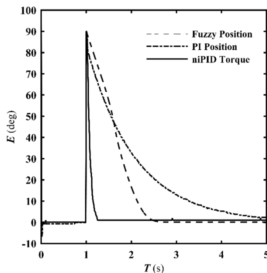
Fig. 14 Controllers position error comparison
