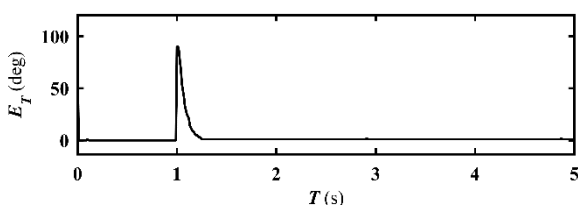
Fig. 12 Position error for fractional order PID torque control
