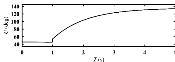
Fig. 9 Control signal for PI controller
