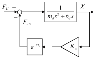
Fig. 1 Block diagram of the haptic device used by Minsky et al.
