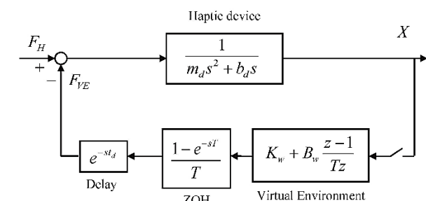
Fig. 2 Block diagram of the haptic device used by Gil et al
