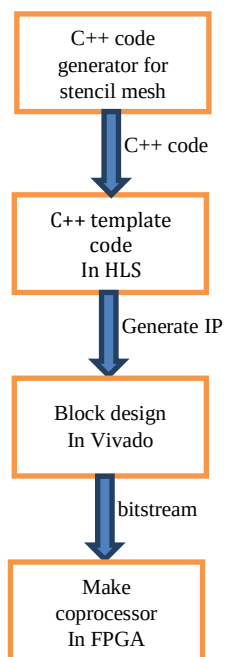
Fig 3 Development of FPGA based coprocessor using the proposed framework
