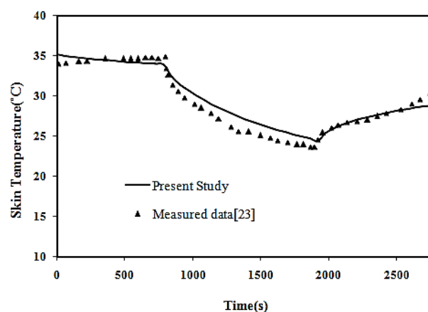
Fig. 4 Comparison of the simulated left hand skin temperature and measured data (Zhang et al [23])
