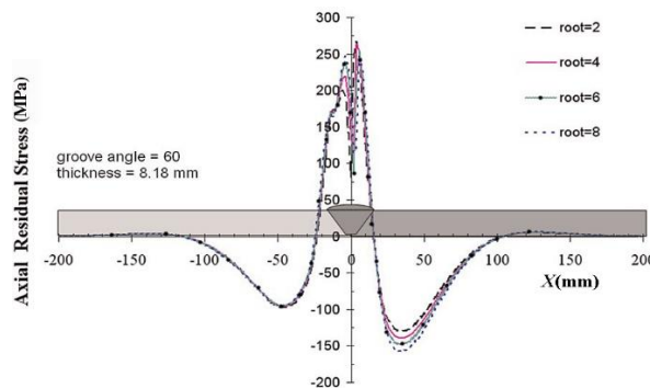
Fig. 13 Axial residual stresses on the inner surface for joints with different root openings
