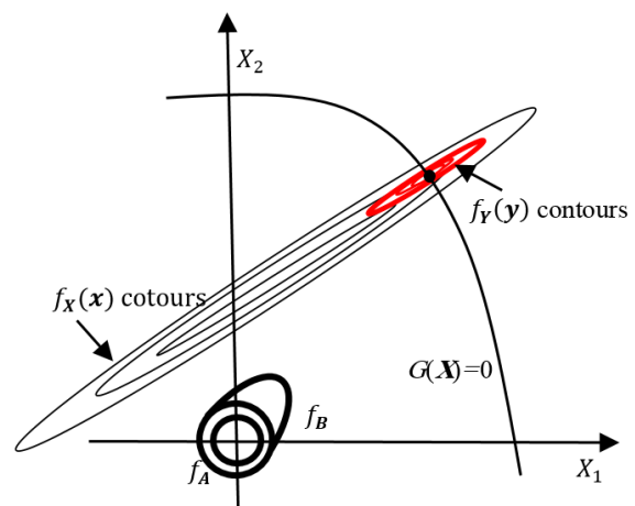
Fig. 2 Importance sampling in directional simulation
