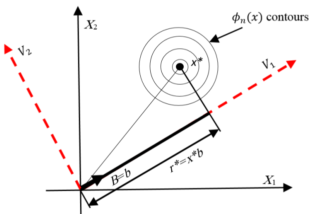
Fig. 3 Integration along B=b in standard Normal space
