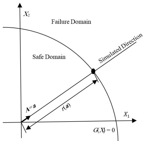
Fig. 1 Directional Simulation
