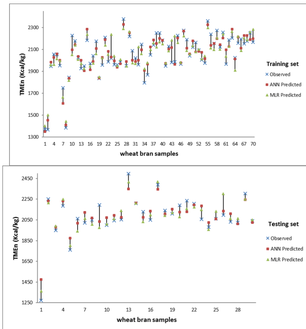
Figure 1. Comparison of observed and model-predicted values for nitrogen-corrected true metabolizable energy (TMEn; Kcal kg -1 DM) of wheat bran samples (n= 100) obtained by Multiple Linear Regression (MLR) and Artificial Neural Network (ANN) models from training (n= 70) and testing (n= 30) data sets.
