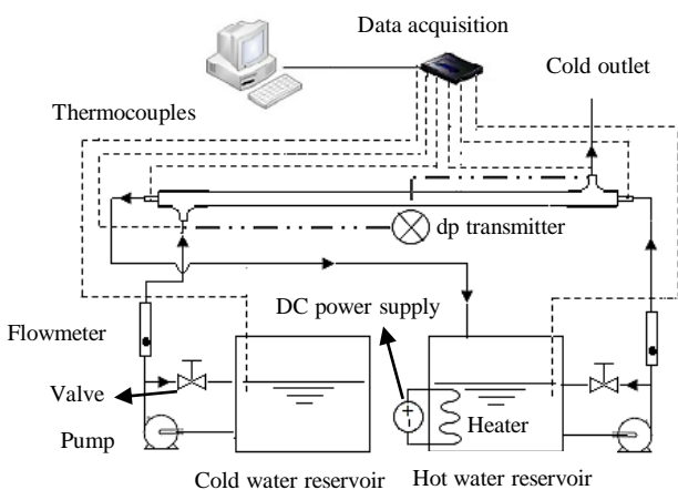
Fig. 2 Schematic of the setup for testing heat transfer coefficient and pressure drop in heat exchanger
