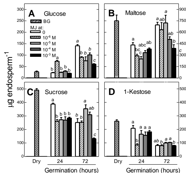
Figure 3. The content of glucose (A), maltose (B), sucrose (C) and 1-kestose (D) in endosperm of triticale kernel before germination (Dry, BG) and after germination for 24 and 72 h at 20°C in the presence of MJ at 0, 10^{-6} , 10^{-5} , 10^{-4} and 10^{-3} M concentration.
