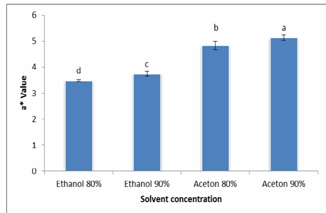
Fig 2 a* value of extracted chlorophyll by different solvents
