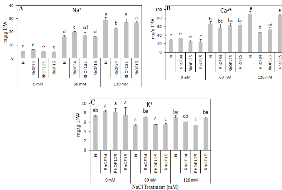
Figure 3. Mineral nutrient accumulation (Na + , Ca 2+ and K + ) in shoots of V. faba inoculated with rhizobial strains. N: Non-inoculated plants. Bars with different letters are significantly different at P \leq 0.05 according to the SNK test.
